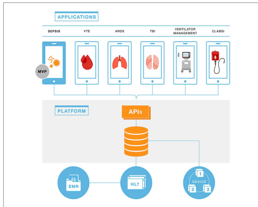
Figure 4 High-level architecture of the CDS tool
